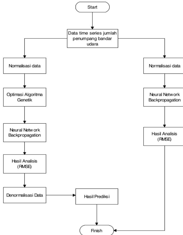
Gambar 4. Model Penerapan Neural Network Berbasis Genetic Algorithm
