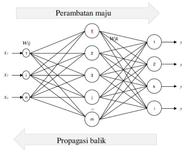
Gambar 2. Arsitektur Neural Network Backpropagation
