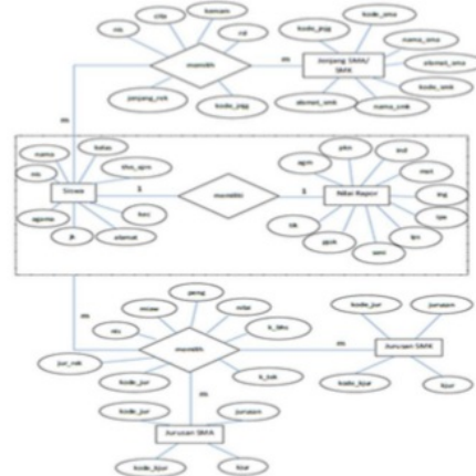
Gambar 12. Entity Relationship Diagram
