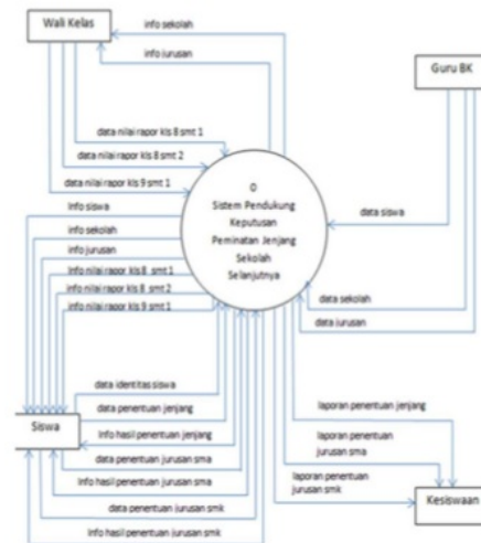
Gambar 5. Context Diagram
