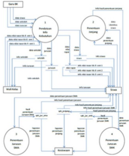
Gambar 7. DFD Level 0
