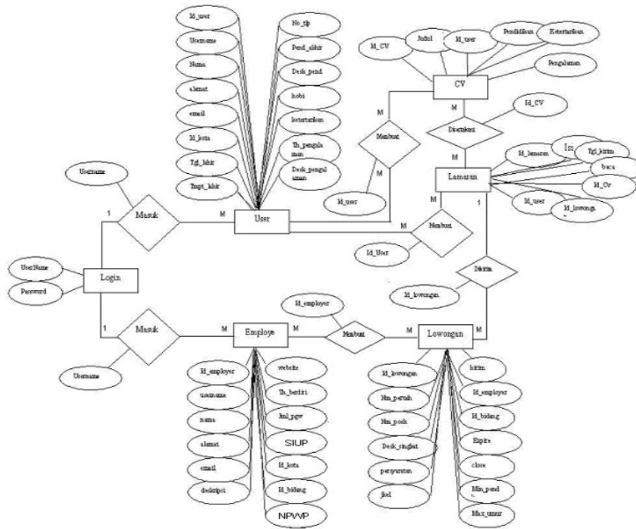
Gambar 8 Entity Relationship Diagram
