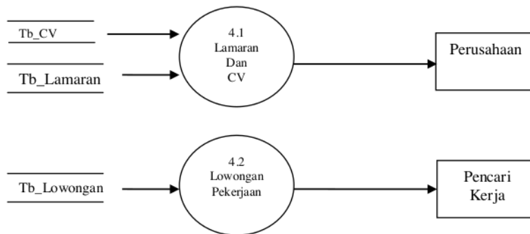
Gambar 7 DFD Level 1 Proses 4
