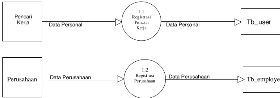
4 Gambar 4 DFD Level 1 Proses 1
