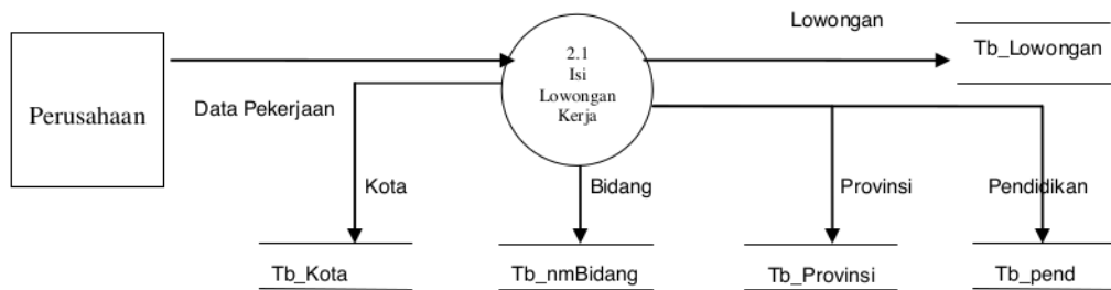
11 Gambar 5 DFD Level 1 Proses 2
