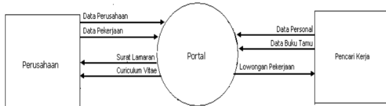
Gambar 1 Context Diagram
