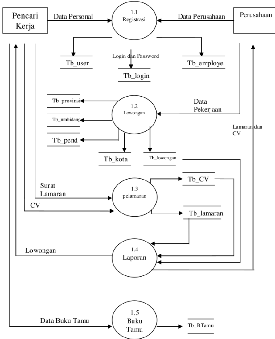
7 Gambar 3 DFD Level 0
