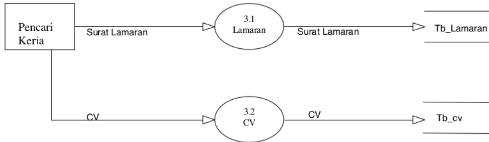
Gambar 6 DFD Level 1 Proses 3
