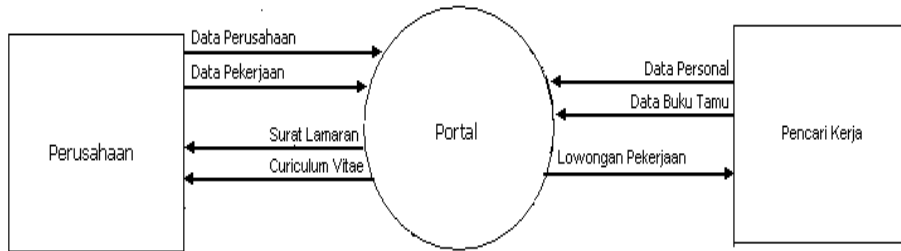
Gambar 1 Context Diagram
