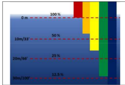
Figure 2: Absorption Of Light By Water
