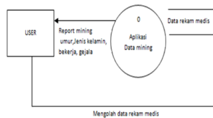
Gambar 1. DFD Level 0
