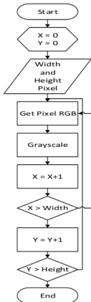
Fig. 3 Grayscale Method
