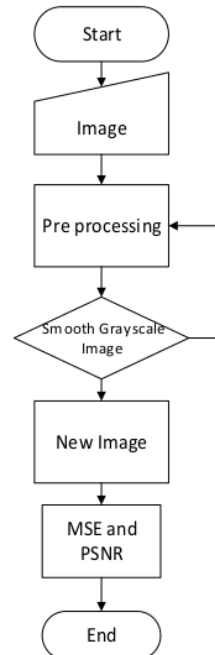
Fig. 1 Methodology Research
