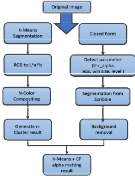
Figure 1. Flowchart of the improved clustering
