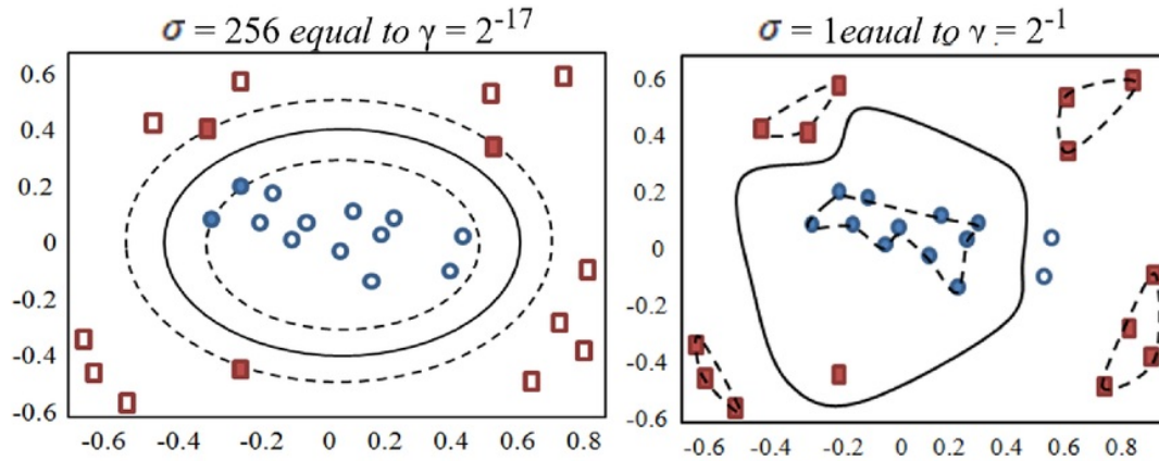
Figure 4. SVM-RBF Kernel Classification for \gamma = 2^{-1} and \gamma = 2^{-17} , ■ ● = feature vector class +1, ○ ● = feature vector class -1, ■ ● = support vector
