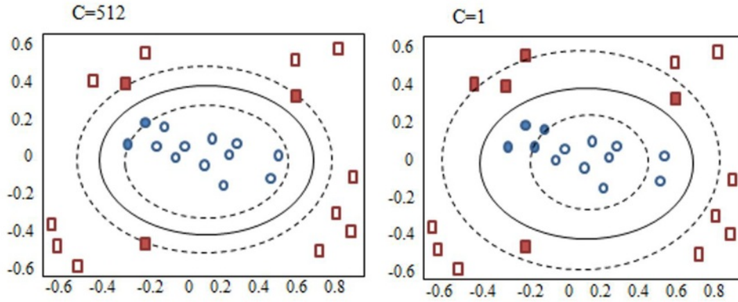
Figure 3. SVM-RBF Kernel Classification for C = 512 and C = 1 , ■ ● = feature vector class +1, ○ ● = feature vector class -1, ■ ● = support vector
