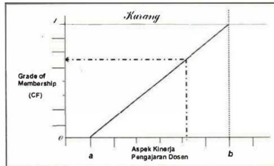
Gambar 1. Representasi Himpunan Fuzzy Kurang
