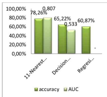
Gambar 3. Perbandingan Kinerja Model Berbasis Backward Elimination
