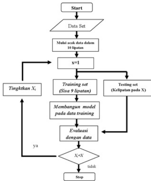
Gambar 2. Flowchart forward selection
