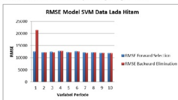
Gambar 6. Grafik RMSE Model SVM Lada Hitam
