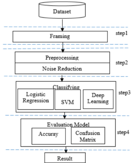
Fig. 2. Gender Recognition Proposed Method.
