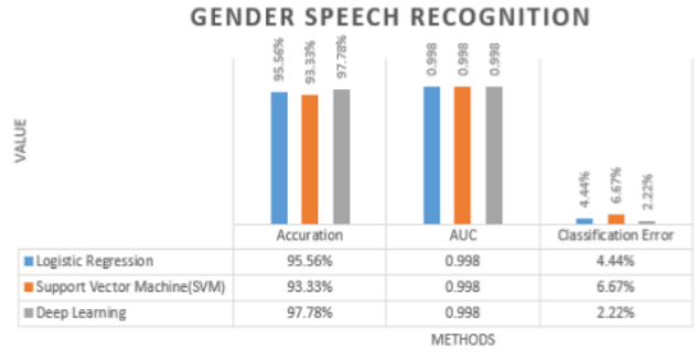
Fig. 3. Comparison of Gender Speech Recognition method.
