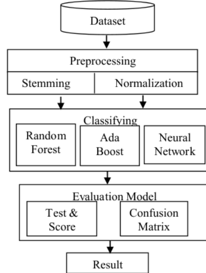
Figure 2 : Hatespeech's Prediction Model
