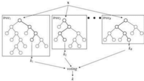
Figure 3 :Random Forest Architecture (Verikas et al.2011)
