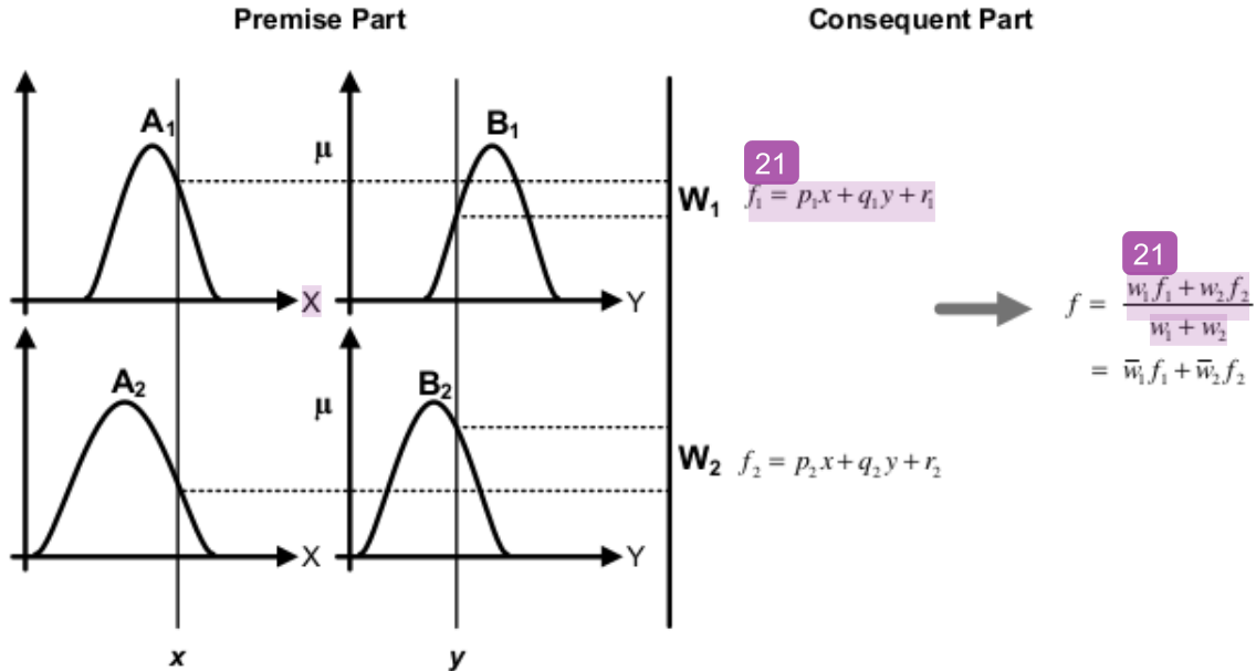
Fig. 1. Fuzzy reasoning mechanism
