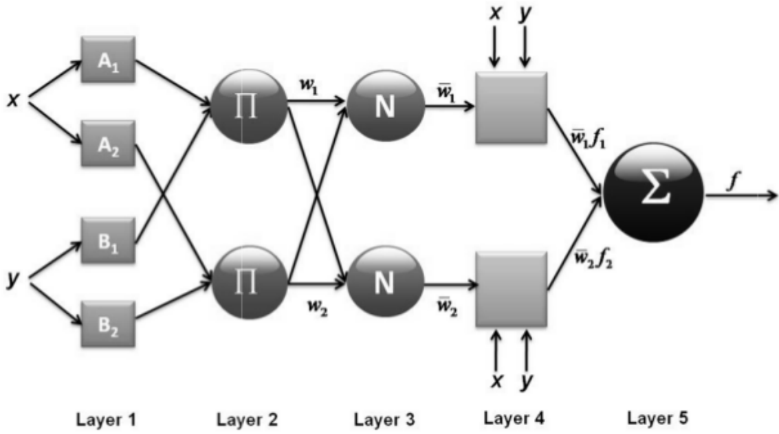
Fig. 2. Adaptive neuro-fuzzy inferences system architecture
