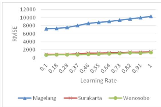
Figure 3. Learning rate adjustment.
