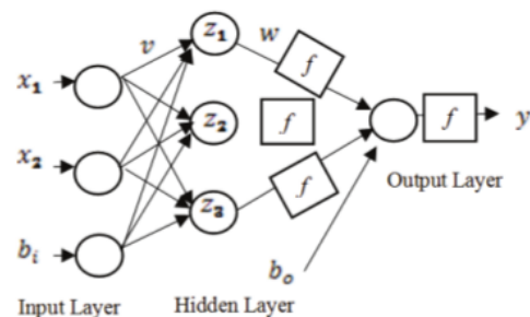
Figure 1. Single hidden layer BPNN.
