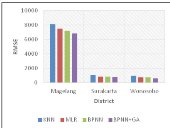
Figure 5. Comparison of BPNN and BPNN+GA.
