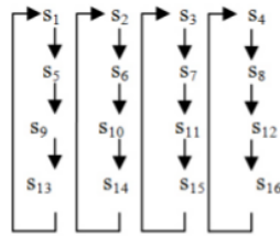
Fig. 11. Illustration Inter-Gatras Odd and Even Sequences
