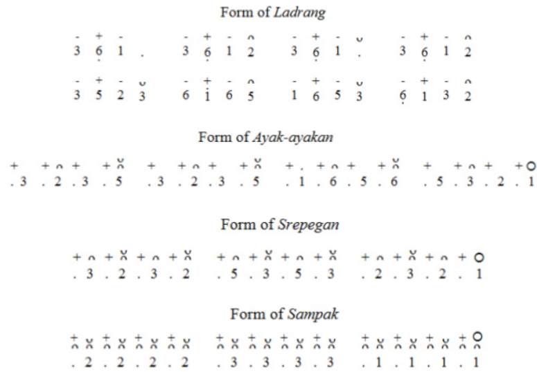
Fig. 1. Forms of Gendings [19]
