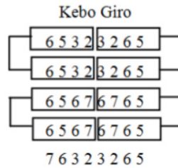
Fig. 6. Identical gattras in gending Kebo Giro
