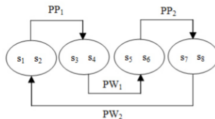
Fig. 10. Illustration of odd and even group sequences
