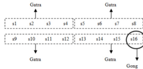
Fig. 5. Structure of gending lancaran
