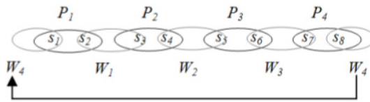
Fig. 8. Illustration of odd and even sequences
