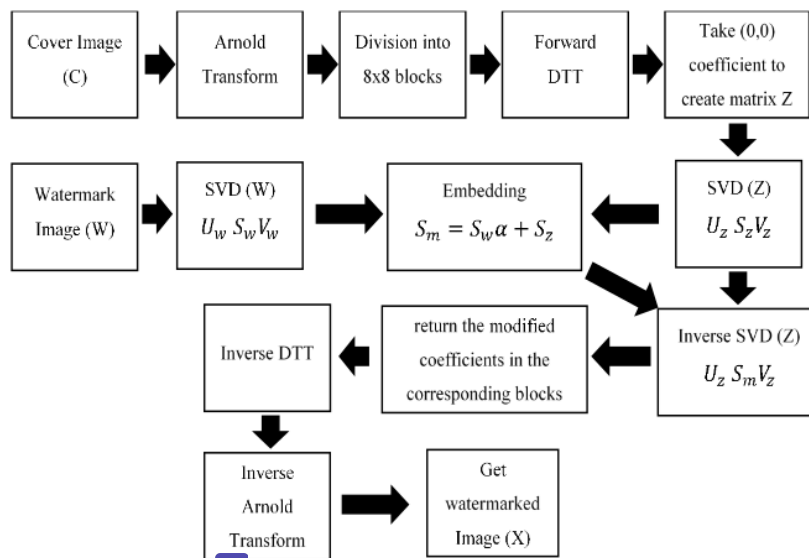
Figure. 1 Watermark embedding procedure
