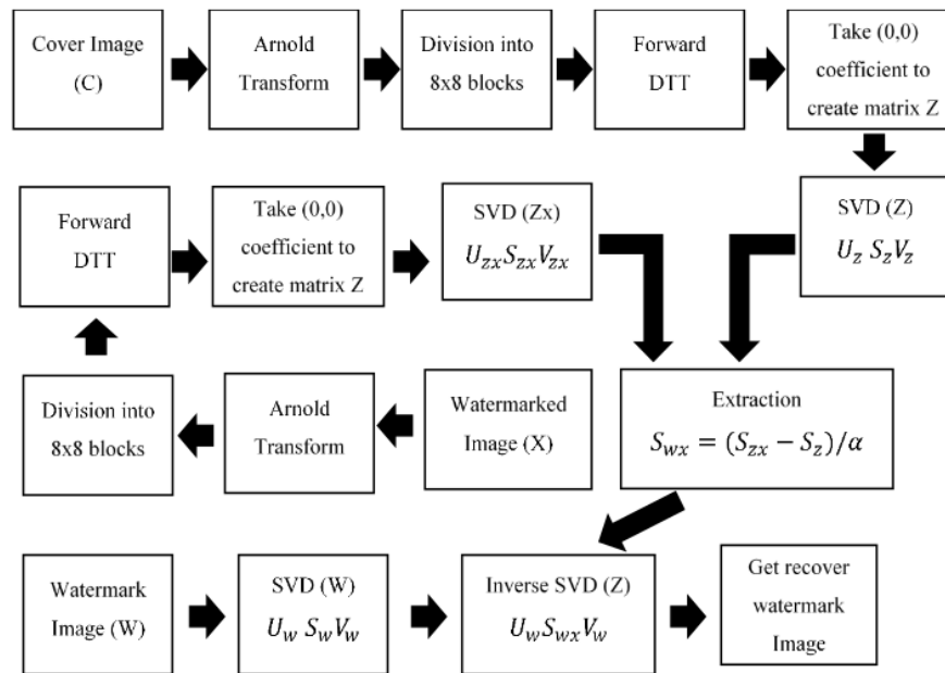
Figure. 2 Watermark extraction procedure
