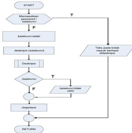
Gambar 7. Gambar proses Dekripsi
