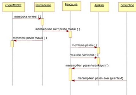
Gambar 5. Sequence Diagram Menerima SMS
