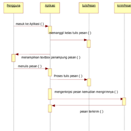
Gambar 4. Diagram Pengiriman SMS
