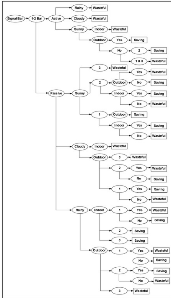
Fig. 2. Decision Tree for signal bar 1-2.
