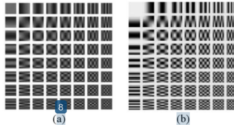
Figure 1. 2-D image base of (a) DTT, (b) DCT
