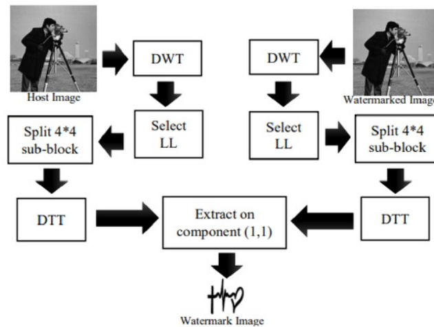
Figure 4. Watermark extraction scheme
