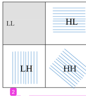
Figure 2. 2-D discrete wavelet transform
