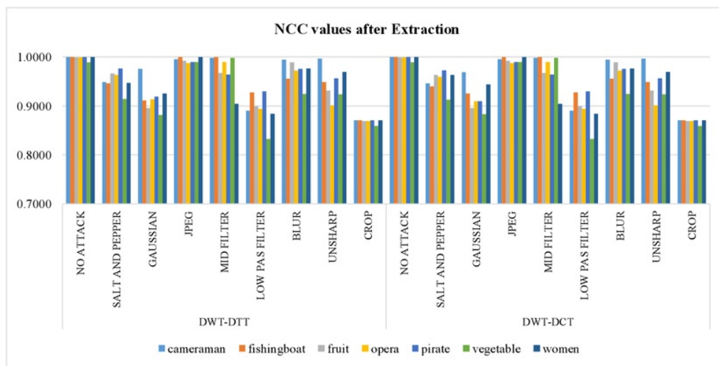
Figure 7. NCC values Chart
