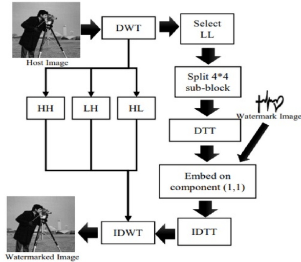
Figure 3. Watermark insertion scheme
