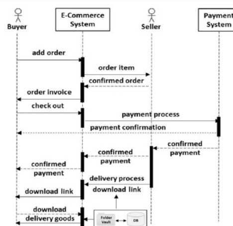
Fig. 1: Folder Vault Sequence Diagram
