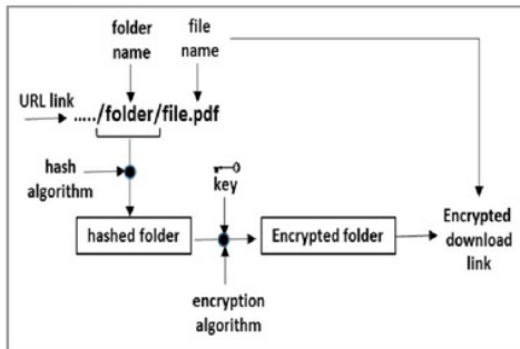
Fig. 3: Download Link Encryption Process
