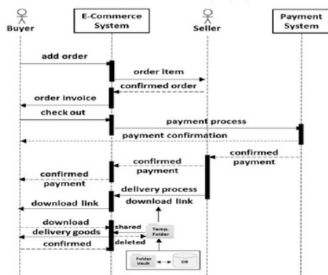
Fig. 8: Download Link with Temporary Folder
