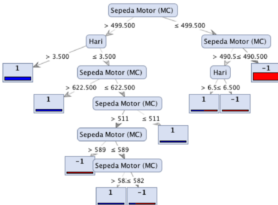
Gambar 6. Eksperimen 4.4.1 : Adaboost model Weight = 3.916
