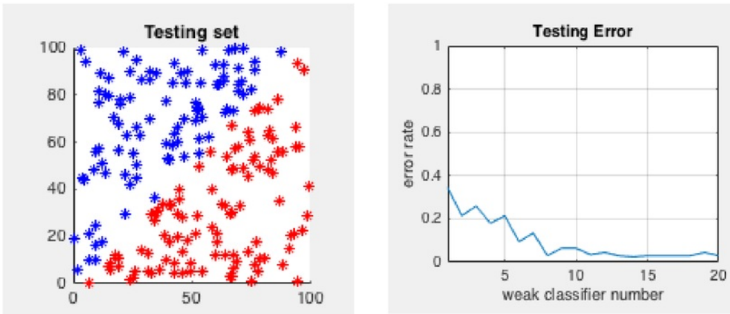
Gambar 3. Result Test Data
